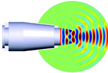
Visualization of the sound directivity generated by an APU exhaust Model courtesy of Airbus
