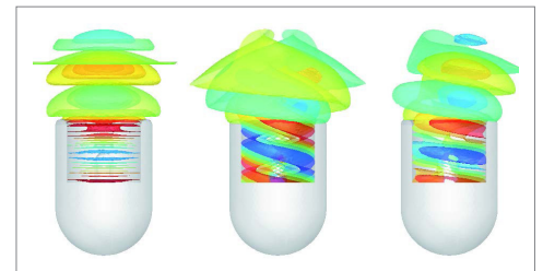
Acoustic modes propagation from engine nacelles
