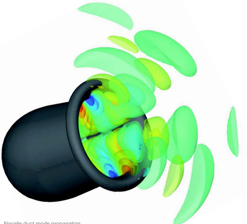
Nacelle duct mode propagation Model courtesy of Alenia Aermacchi
