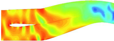
Influence of a splitter within a bypass duct Model courtesy of Airbus
